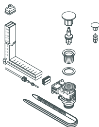
■ Clou downpipe system with leverage for sanitary basins for version without overflow drilling.
