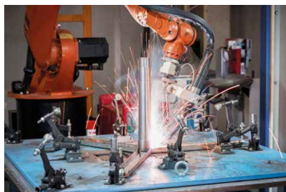
Robot welding
