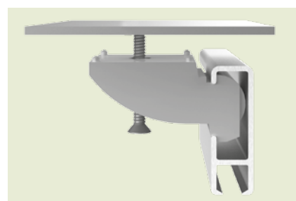
Ceiling bracket - ceiling fixing detail
