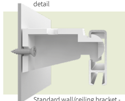
Standard wall/ceiling bracket - wall fixing detail
