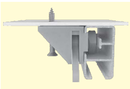
Ceiling bracket - ceiling fixing detail
