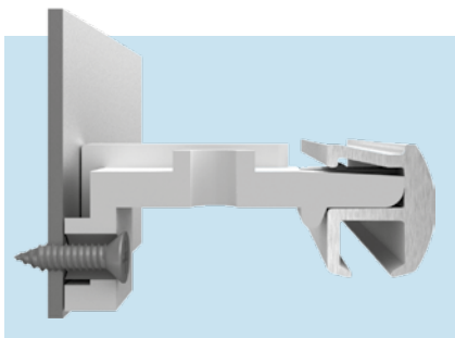
Standard wall/ceiling bracket - wall fixing detail
