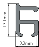
Mini-Optimal profile 4mm groove
