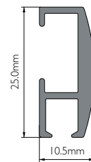
Professional profile 4mm groove
