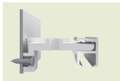
Wall/ceiling bracket - wall fixing detail
