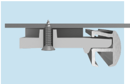
Ceiling bracket - ceiling fixing detail
