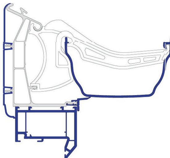
Global eaves beam assembly
