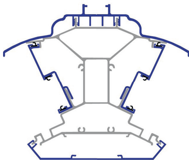
fixed ridge assembly
