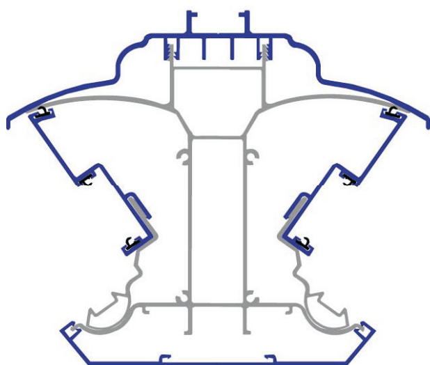
variable ridge assembly
