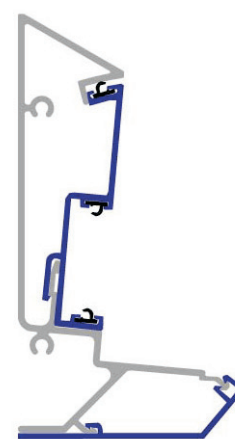
fixed wall plate assembly
